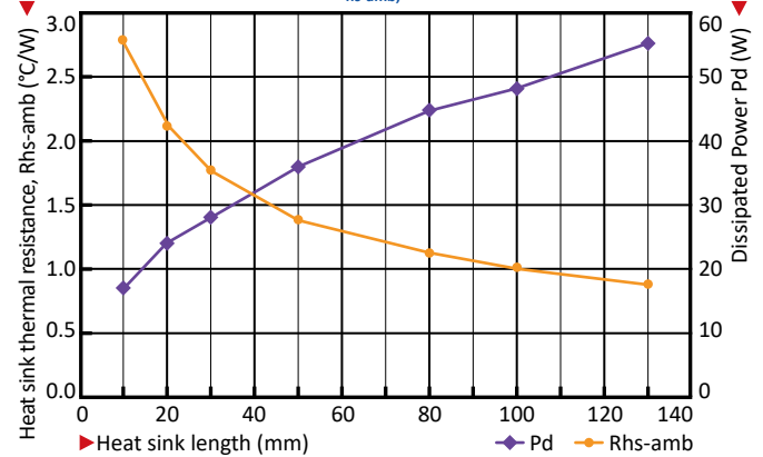
ModuLED Xtra performance data at a heat sink to ambient temperature difference, ΔT hs-amb , of 50 °C
