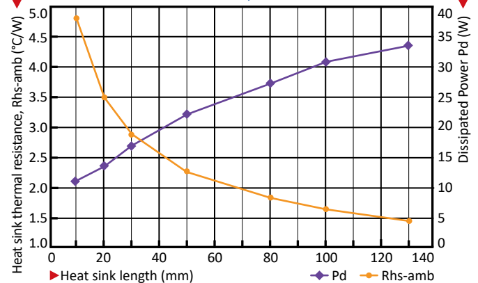
ModuLED Nano performance data at a heat sink to ambient temperature difference, ΔT hs-amb , of 50 °C
