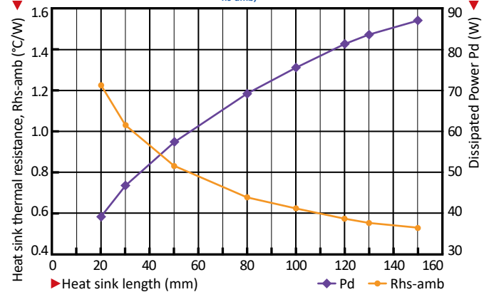
ModuLED Mega performance data at a heat sink to ambient temperature difference, ΔT hs-amb , of 50 °C
