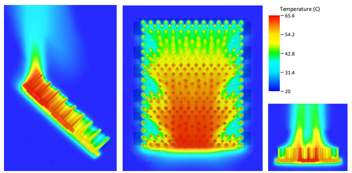
CoolBlock® thermal simulations results CFD
