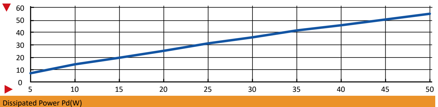
Heat sink to ambient temperature rise T_{hs-amb} (°C)
